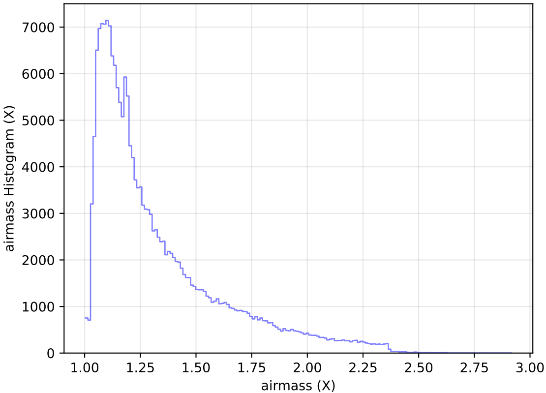
too_elab_r64_d3_ugrizy_v3.4_10yrs All sky g band: airmass Histogram
