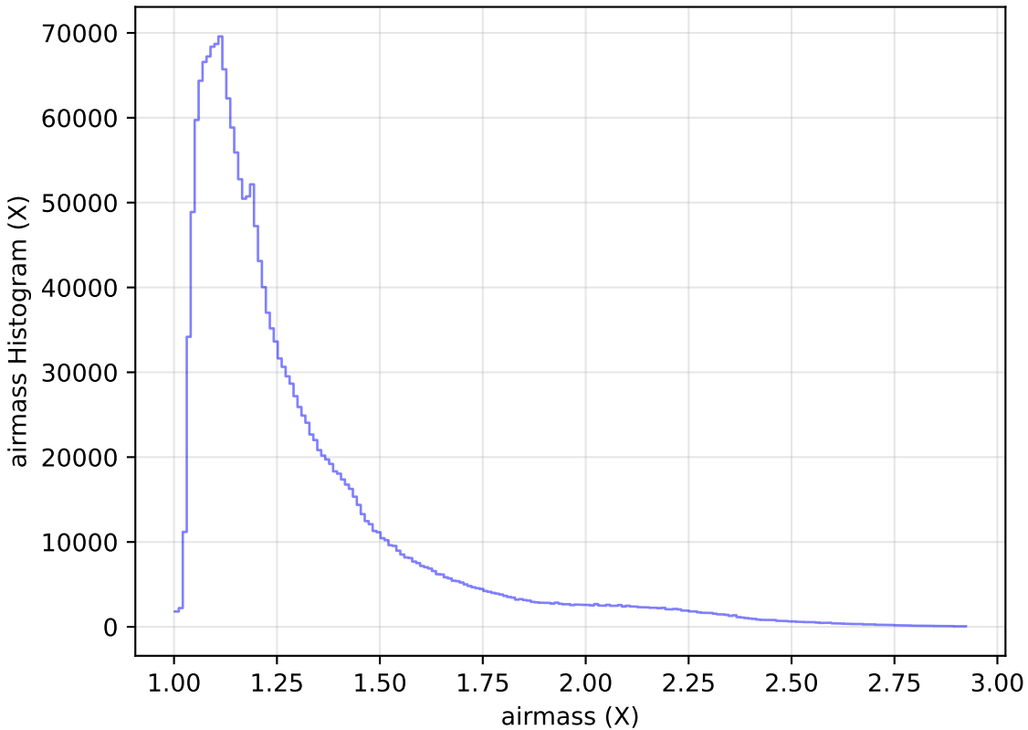
too_elab_r64_d3_ugrizy_v3.4_10yrs All sky all bands: airmass Histogram
