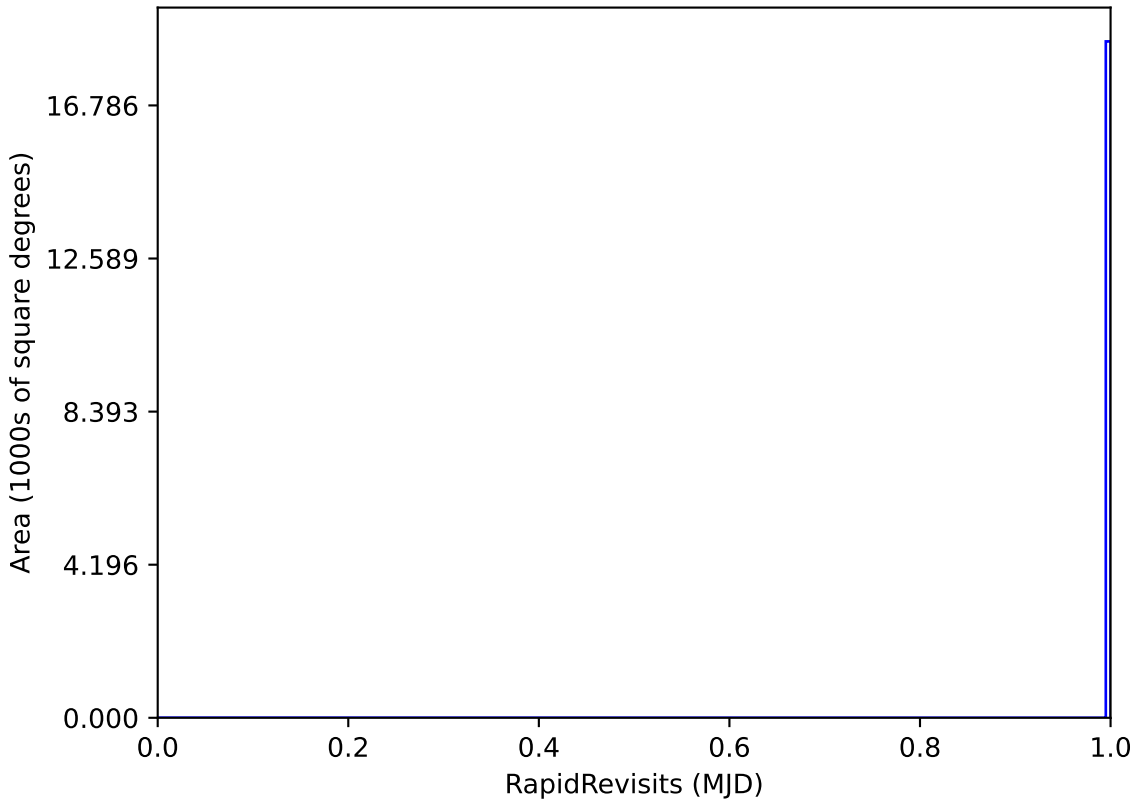
too_elab_r64_d3_ugrizy_v3.4_10yrs WFD: RapidRevisits
