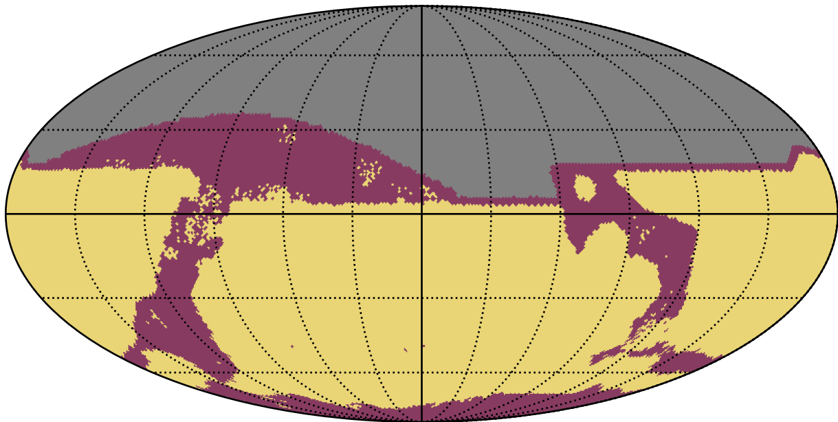
too_elab_r64_d3_ugrizy_v3.4_10yrs All sky: RapidRevisits
