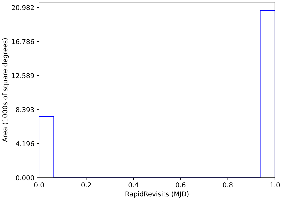
too_elab_r64_d3_ugrizy_v3.4_10yrs All sky: RapidRevisits
