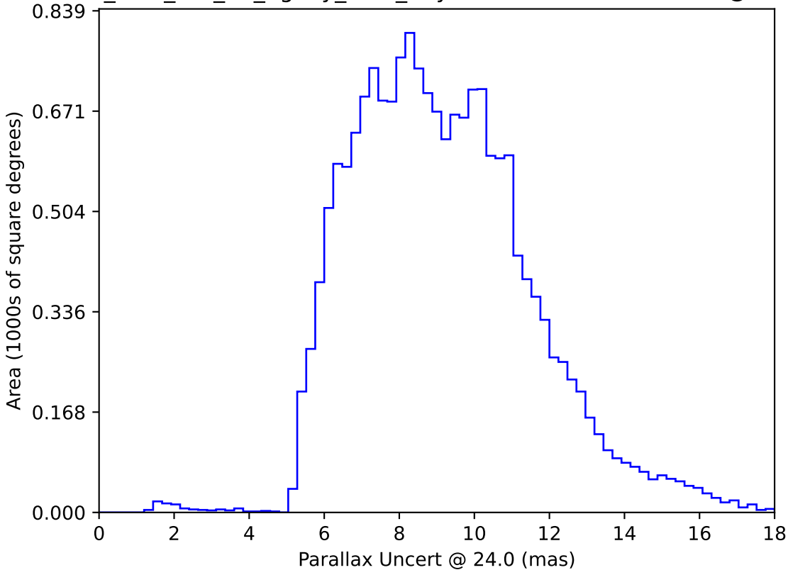
too_elab_r64_d3_ugrizy_v3.4_10yrs WFD: Parallax Uncert @ 24.0
