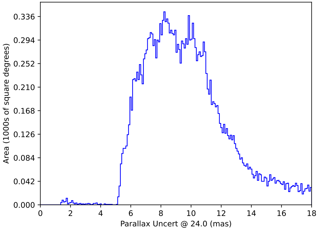
too_elab_r64_d3_ugrizy_v3.4_10yrs All sky: Parallax Uncert @ 24.0
