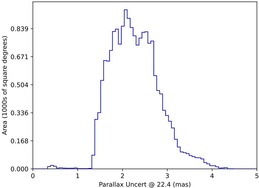
too_elab_r64_d3_ugrizy_v3.4_10yrs WFD: Parallax Uncert @ 22.4
