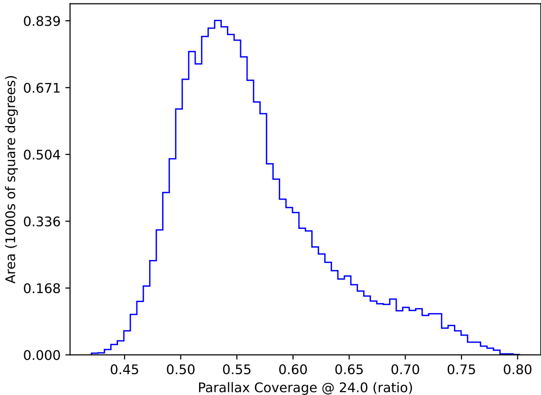
too_elab_r64_d3_ugrizy_v3.4_10yrs WFD: Parallax Coverage @ 24.0
