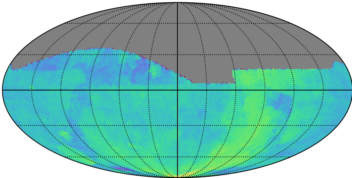
too_elab_r64_d3_ugrizy_v3.4_10yrs All sky: Parallax Coverage @ 24.0
