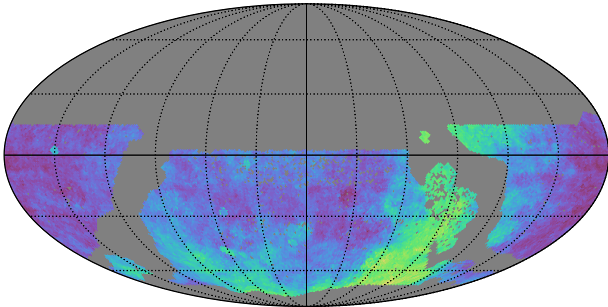
too_elab_r64_d3_ugrizy_v3.4_10yrs WFD: Parallax Coverage @ 22.4
