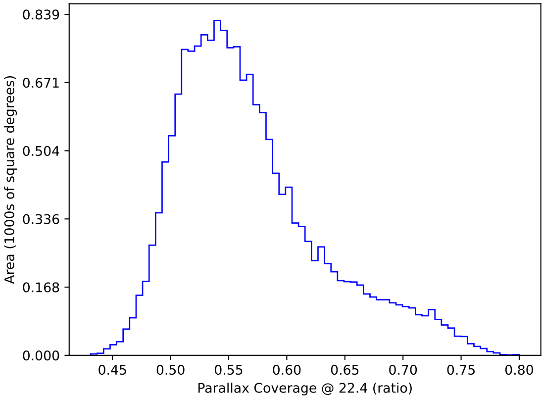
too_elab_r64_d3_ugrizy_v3.4_10yrs WFD: Parallax Coverage @ 22.4
