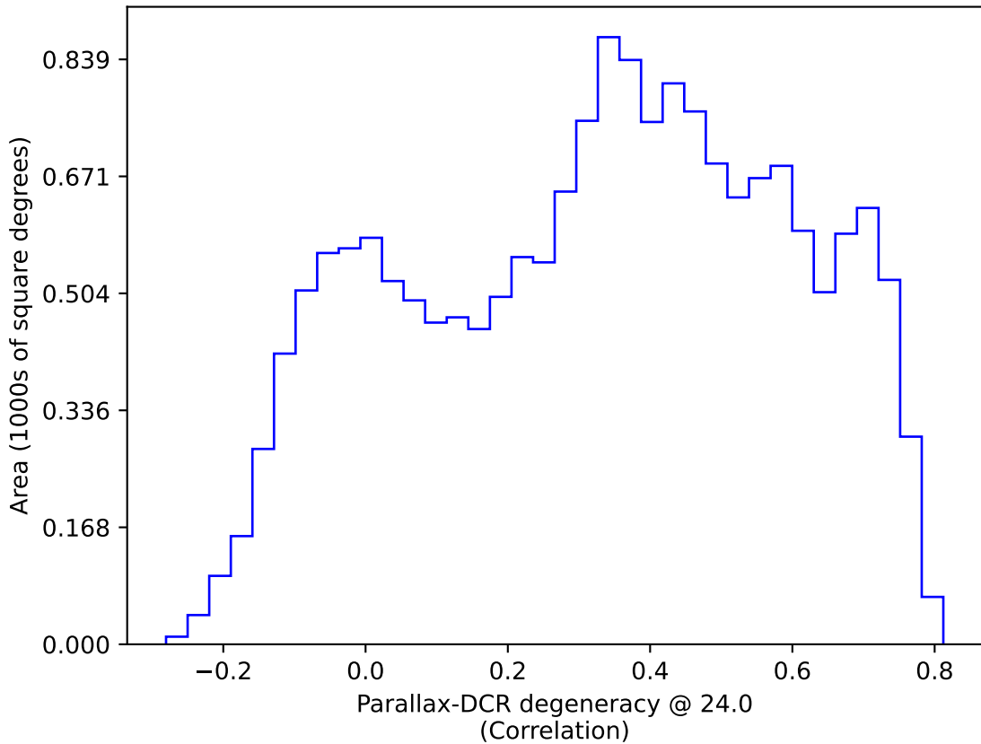
too_elab_r64_d3_ugrizy_v3.4_10yrs WFD: Parallax-DCR degeneracy @ 24.0
