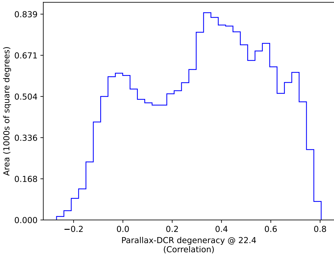
too_elab_r64_d3_ugrizy_v3.4_10yrs WFD: Parallax-DCR degeneracy @ 22.4
