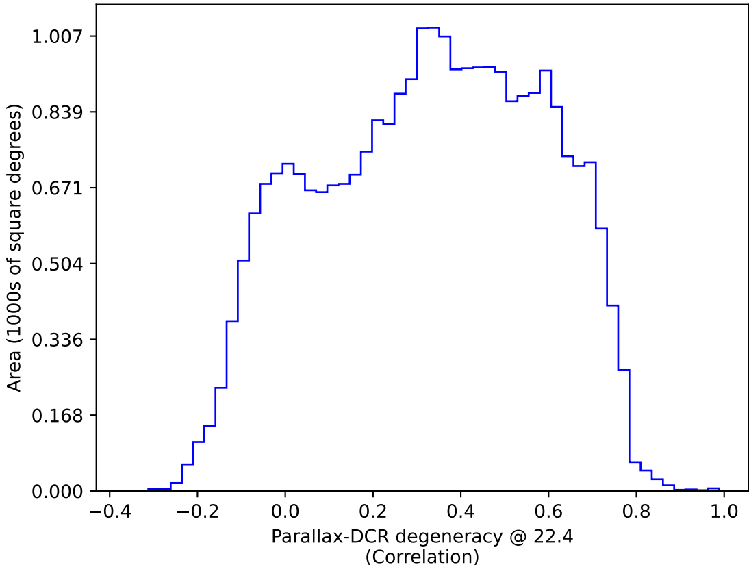
too_elab_r64_d3_ugrizy_v3.4_10yrs All sky: Parallax-DCR degeneracy @ 22.4
