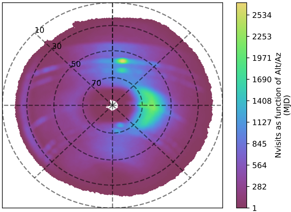
too_elab_r64_d3_ugrizy_v3.4_10yrs r band: Nvisits as function of Alt/Az
