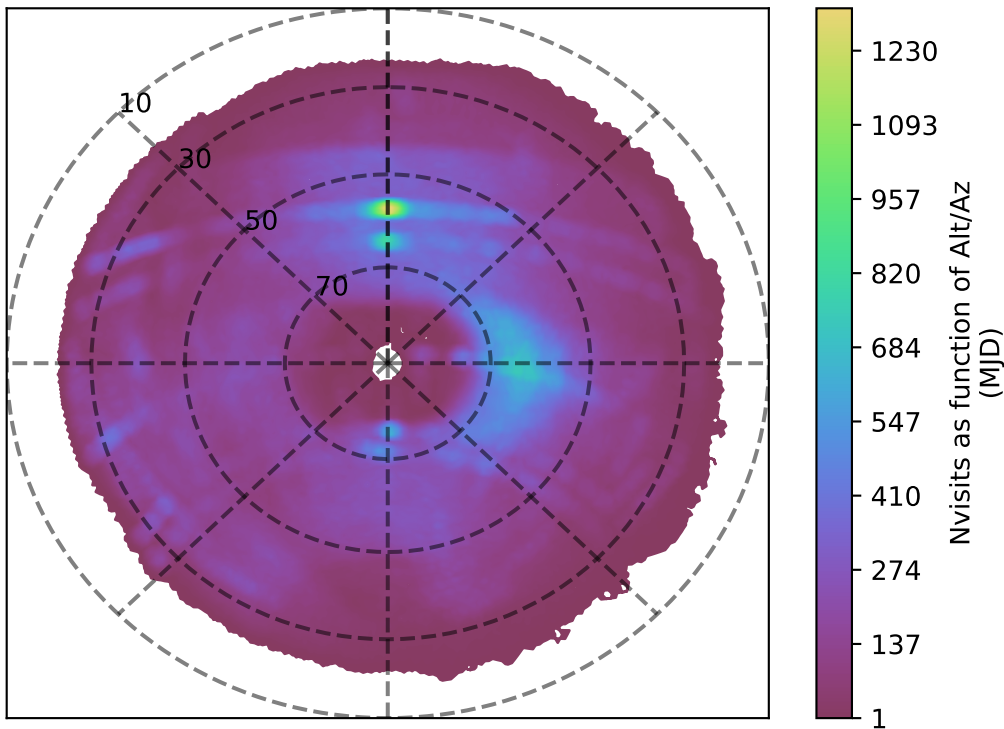
too_elab_r64_d3_ugrizy_v3.4_10yrs g band: Nvisits as function of Alt/Az
