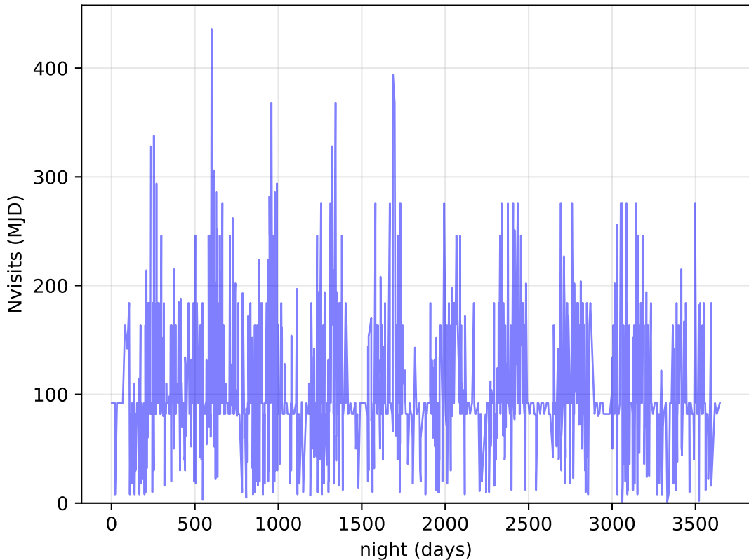
too_elab_r64_d3_ugrizy_v3.4_10yrs DDF: Nvisits
