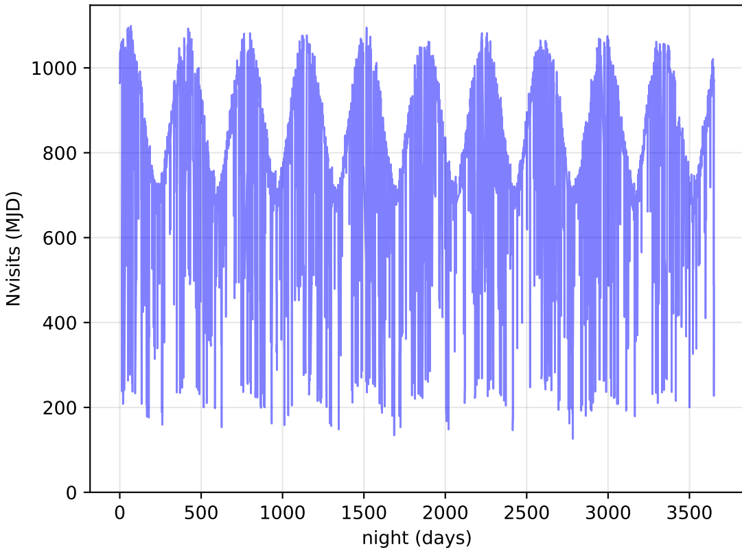
too_elab_r64_d3_ugrizy_v3.4_10yrs All visits: Nvisits
