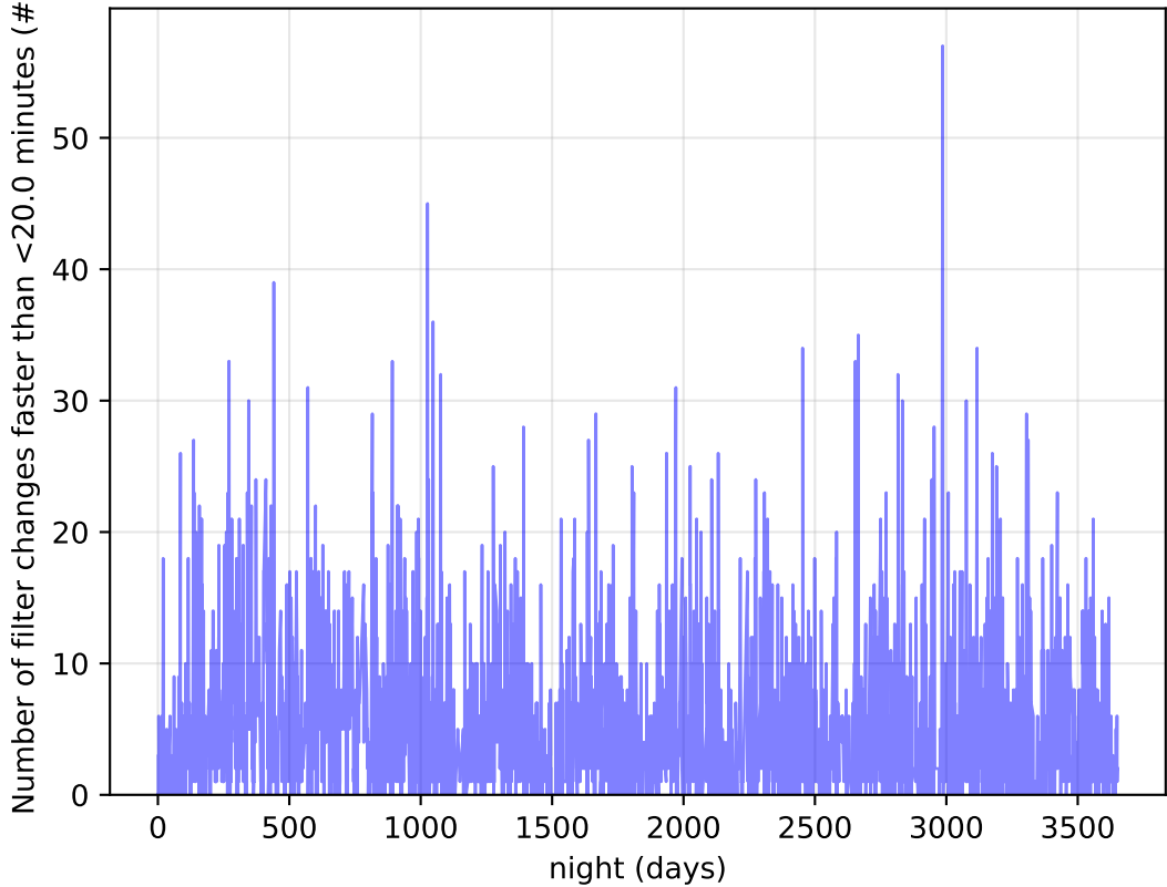
too_elab_r64_d3_ugrizy_v3.4_10yrs Per Night: Number of filter changes faster than <20.0 minutes
