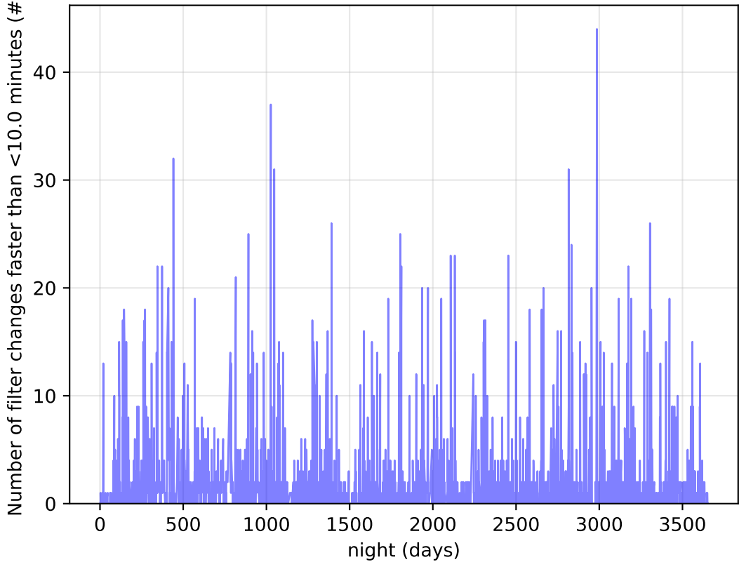
too_elab_r64_d3_ugrizy_v3.4_10yrs Per Night: Number of filter changes faster than <10.0 minutes
