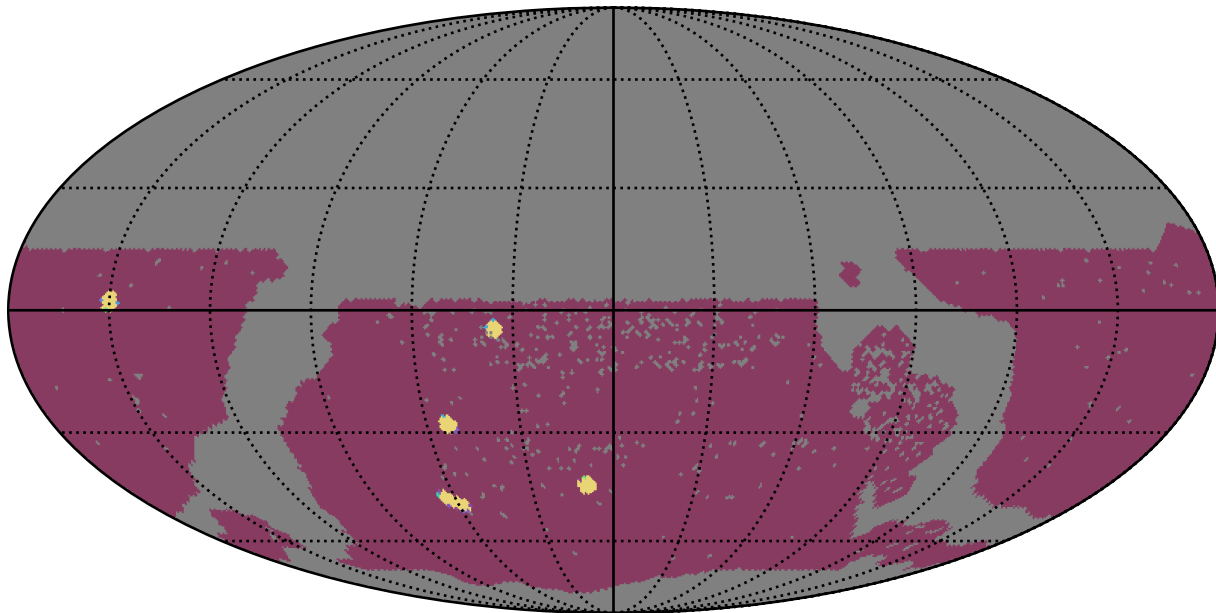
too_elab_r64_d3_ugrizy_v3.4_10yrs WFD: NumberOfQuickRevisits
