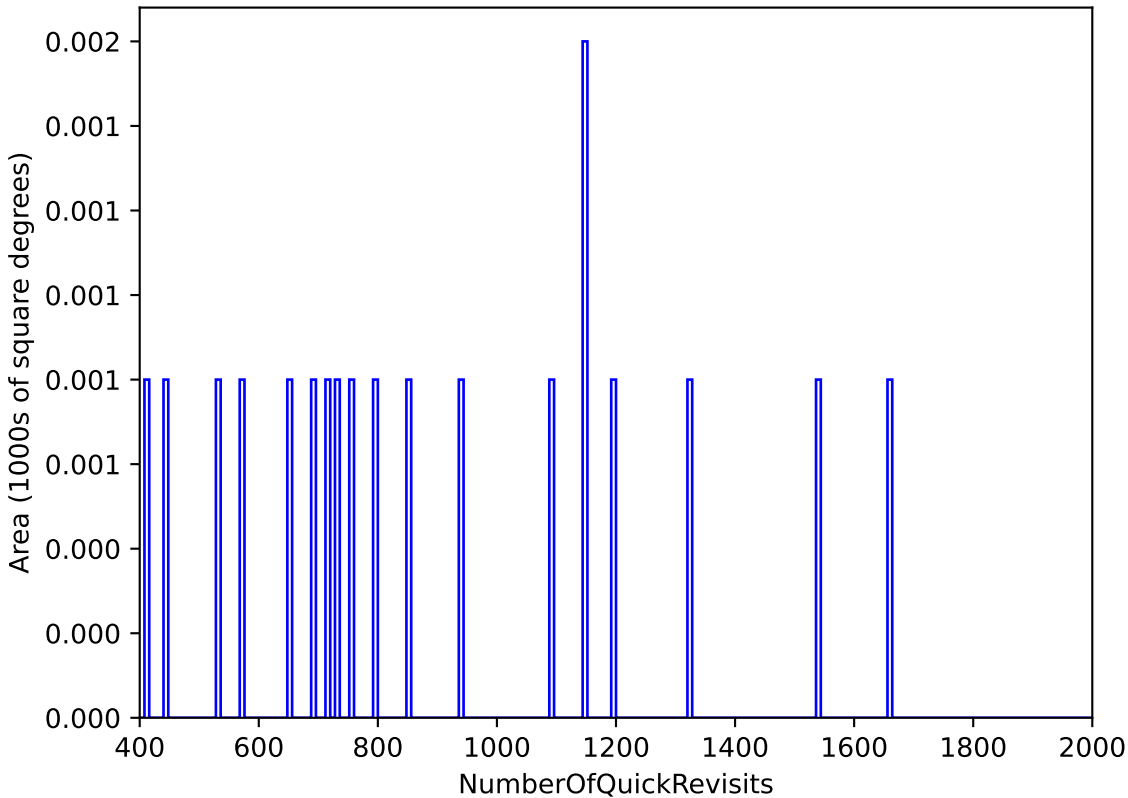
too_elab_r64_d3_ugrizy_v3.4_10yrs WFD: NumberOfQuickRevisits
