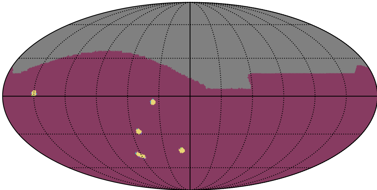
too_elab_r64_d3_ugrizy_v3.4_10yrs All sky: NumberOfQuickRevisits
