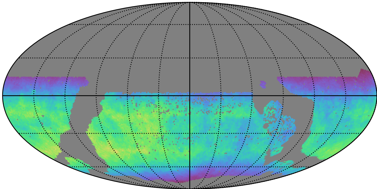
too_elab_r64_d3_ugrizy_v3.4_10yrs WFD y band: Normalized Teff
