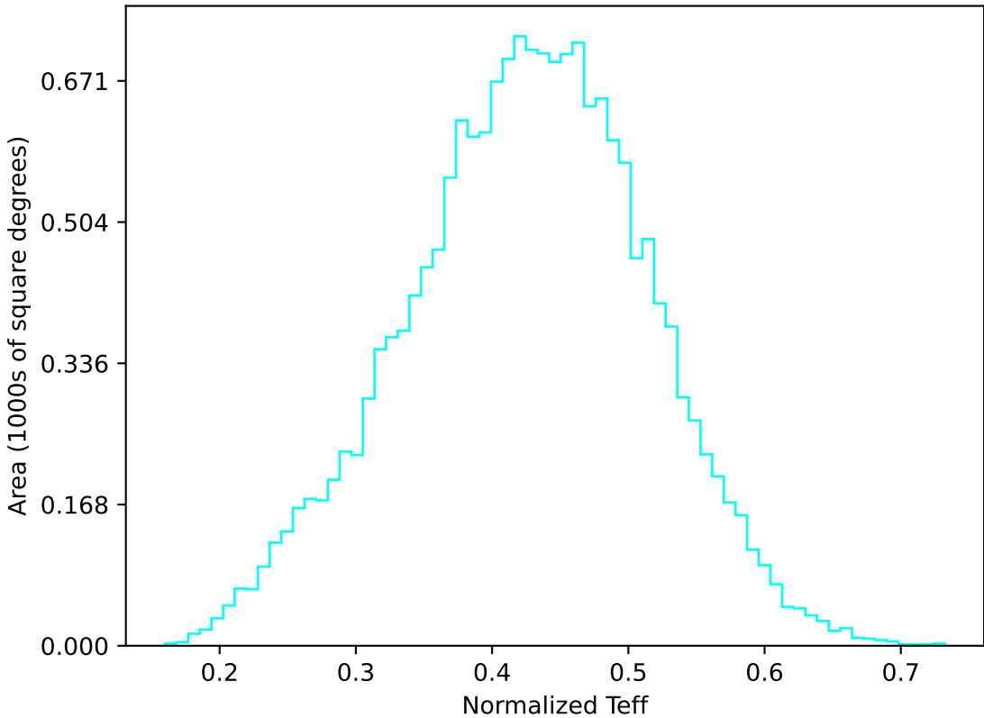
too_elab_r64_d3_ugrizy_v3.4_10yrs WFD u band: Normalized Teff
