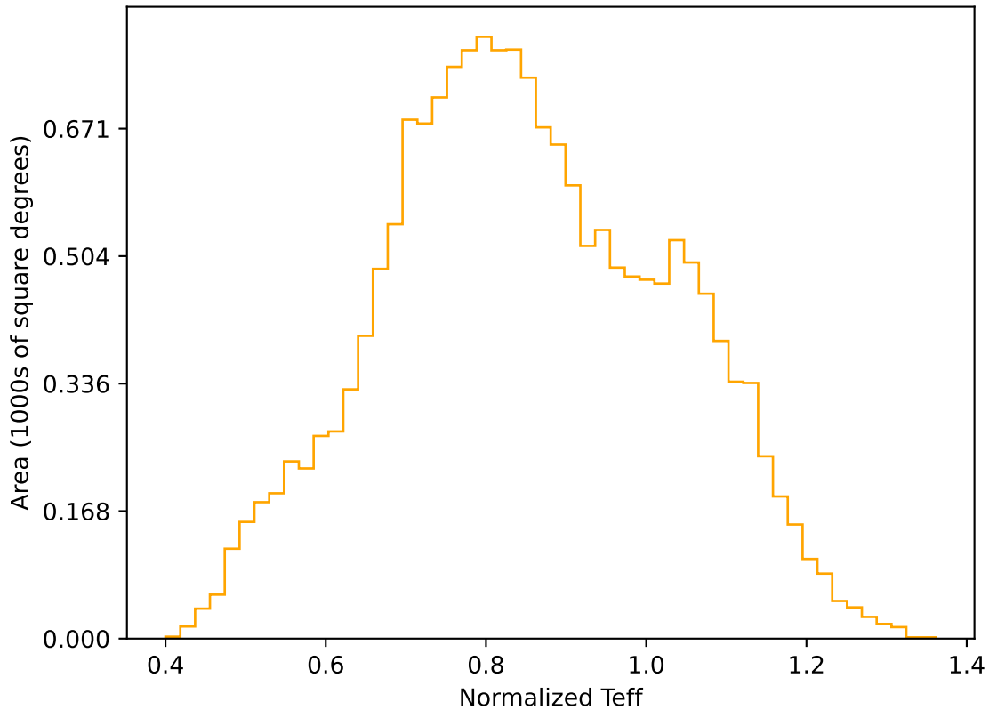
too_elab_r64_d3_ugrizy_v3.4_10yrs WFD r band: Normalized Teff
