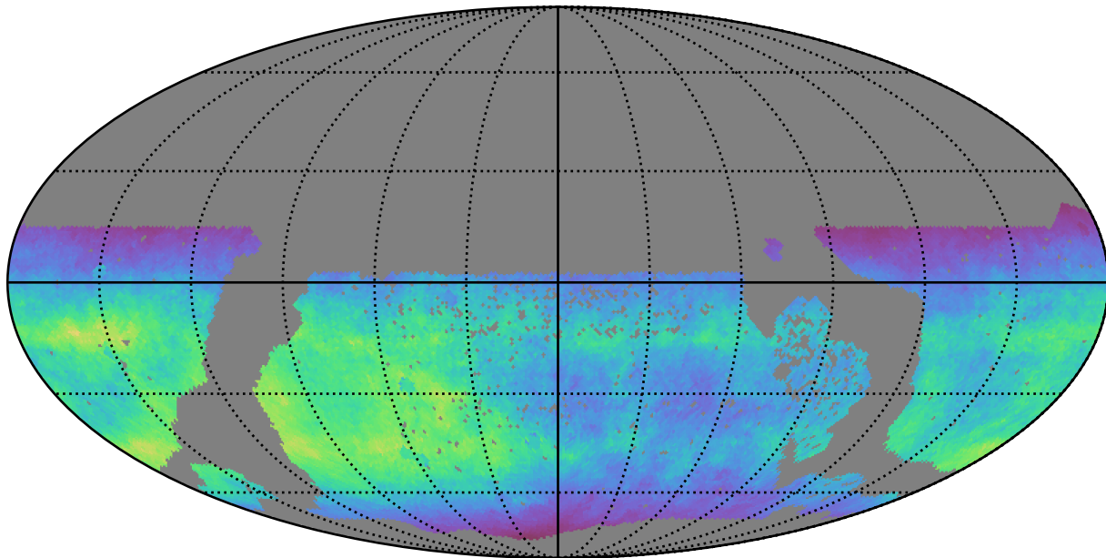
too_elab_r64_d3_ugrizy_v3.4_10yrs WFD i band: Normalized Teff
