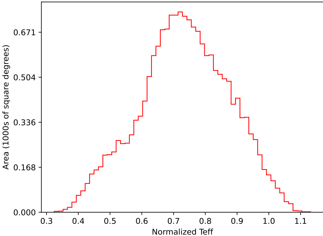
too_elab_r64_d3_ugrizy_v3.4_10yrs WFD i band: Normalized Teff
