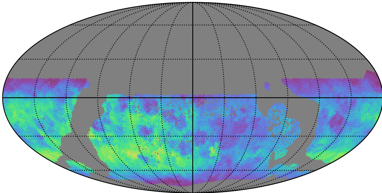
too_elab_r64_d3_ugrizy_v3.4_10yrs WFD g band: Normalized Teff
