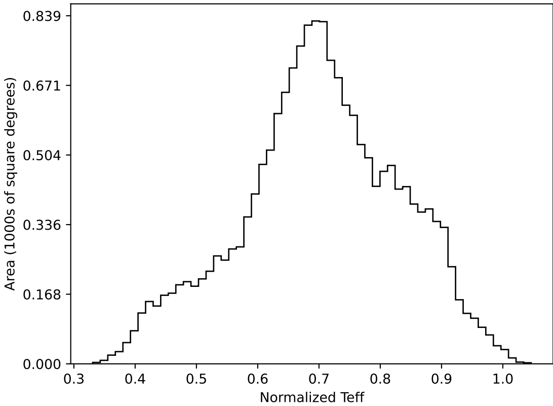
too_elab_r64_d3_ugrizy_v3.4_10yrs WFD all bands: Normalized Teff
