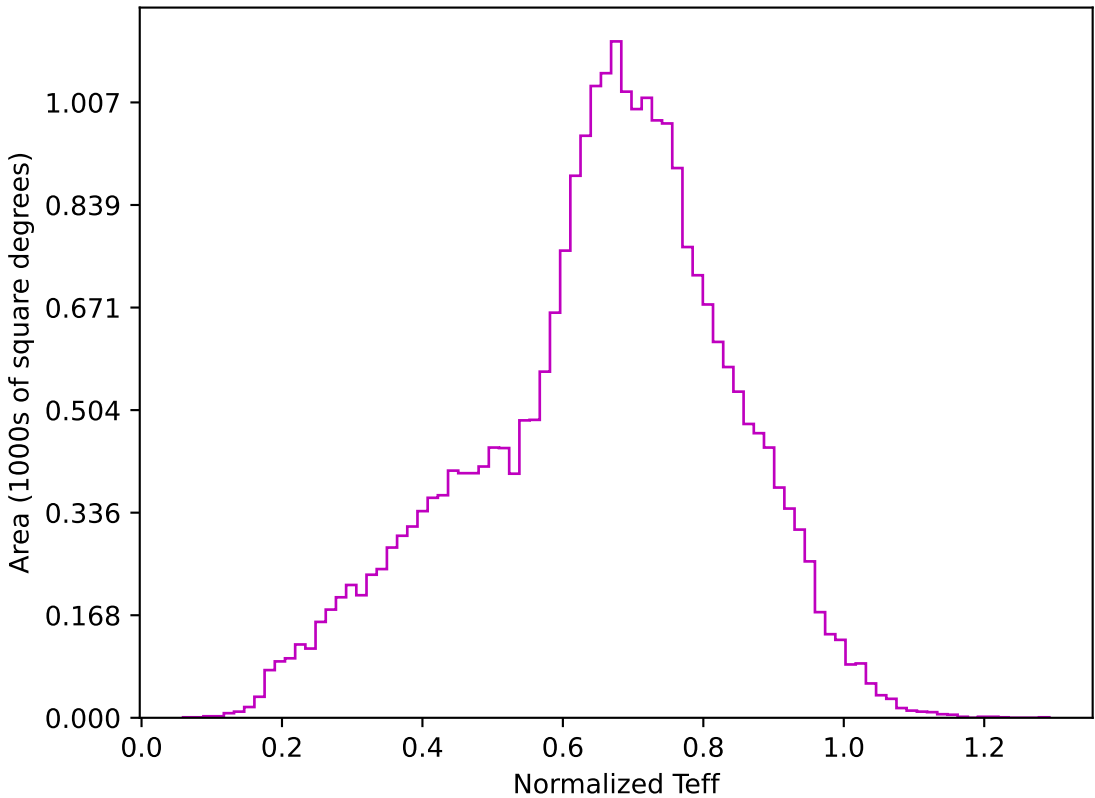
too_elab_r64_d3_ugrizy_v3.4_10yrs All sky z band: Normalized Teff
