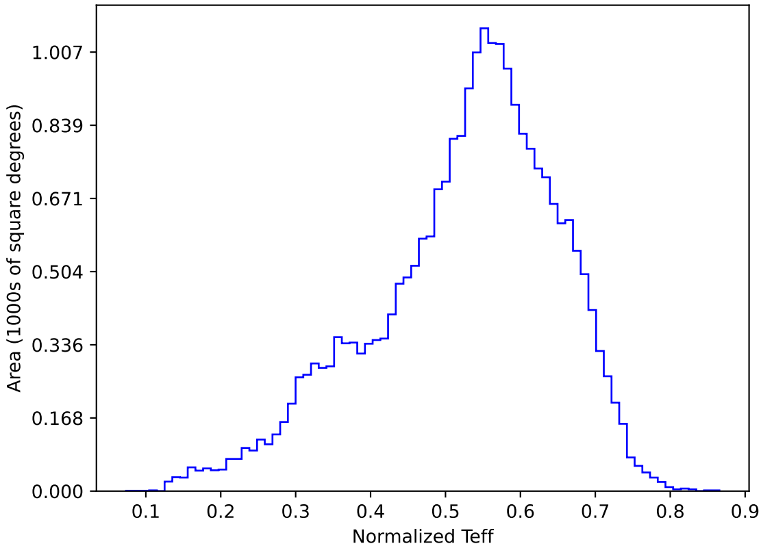
too_elab_r64_d3_ugrizy_v3.4_10yrs All sky y band: Normalized Teff
