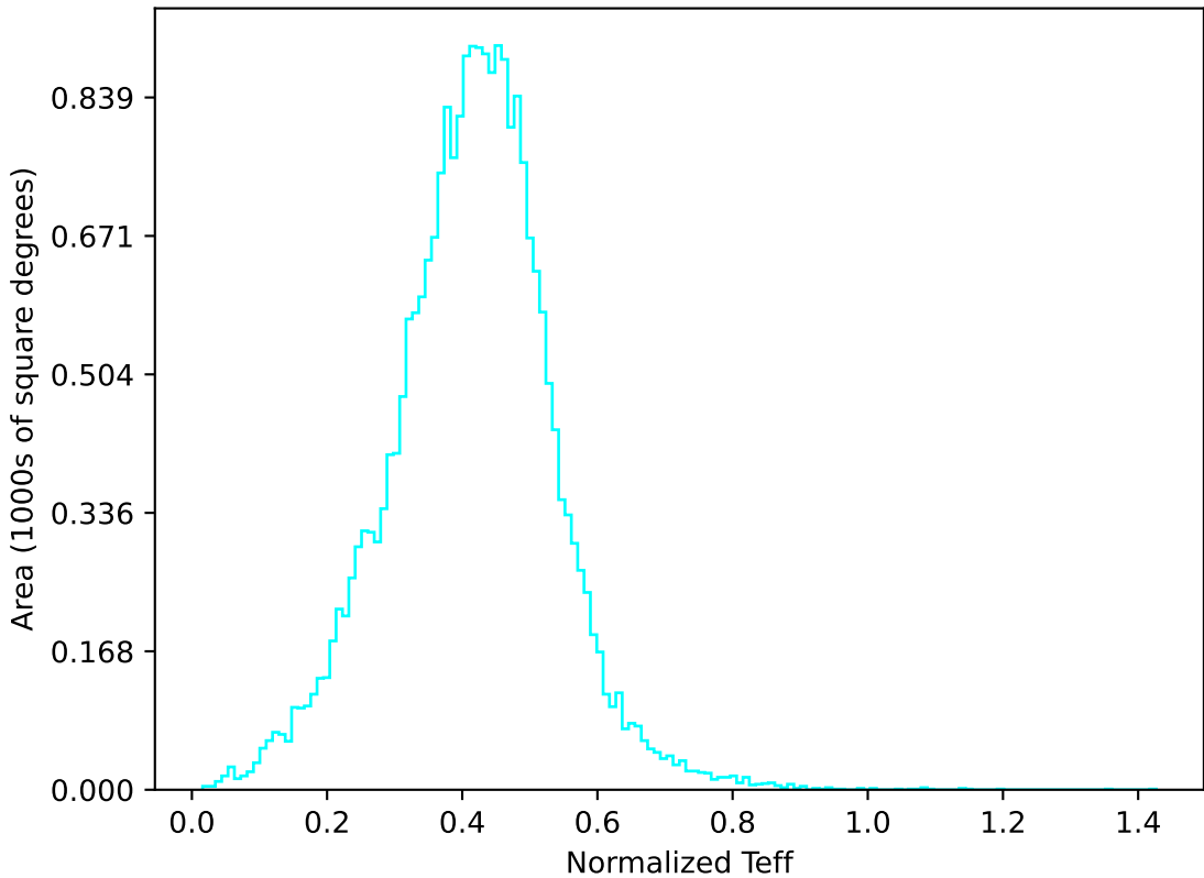
too_elab_r64_d3_ugrizy_v3.4_10yrs All sky u band: Normalized Teff
