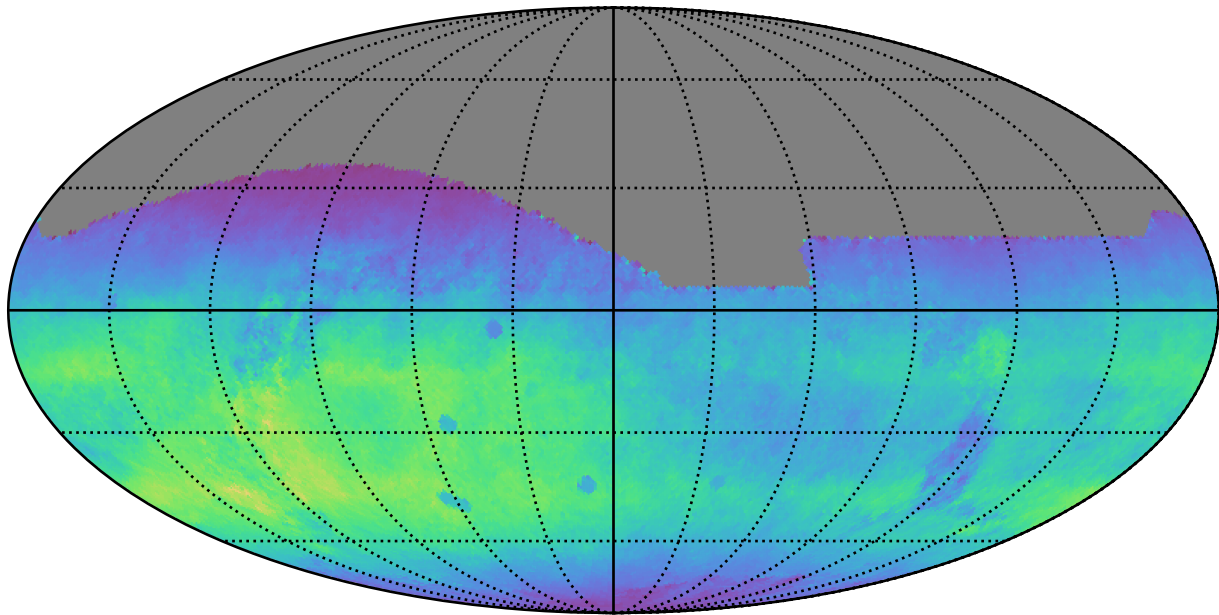
too_elab_r64_d3_ugrizy_v3.4_10yrs All sky r band: Normalized Teff
