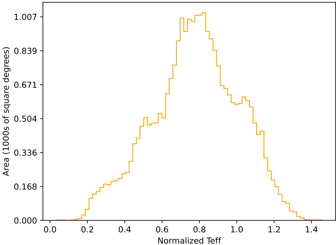
too_elab_r64_d3_ugrizy_v3.4_10yrs All sky r band: Normalized Teff
