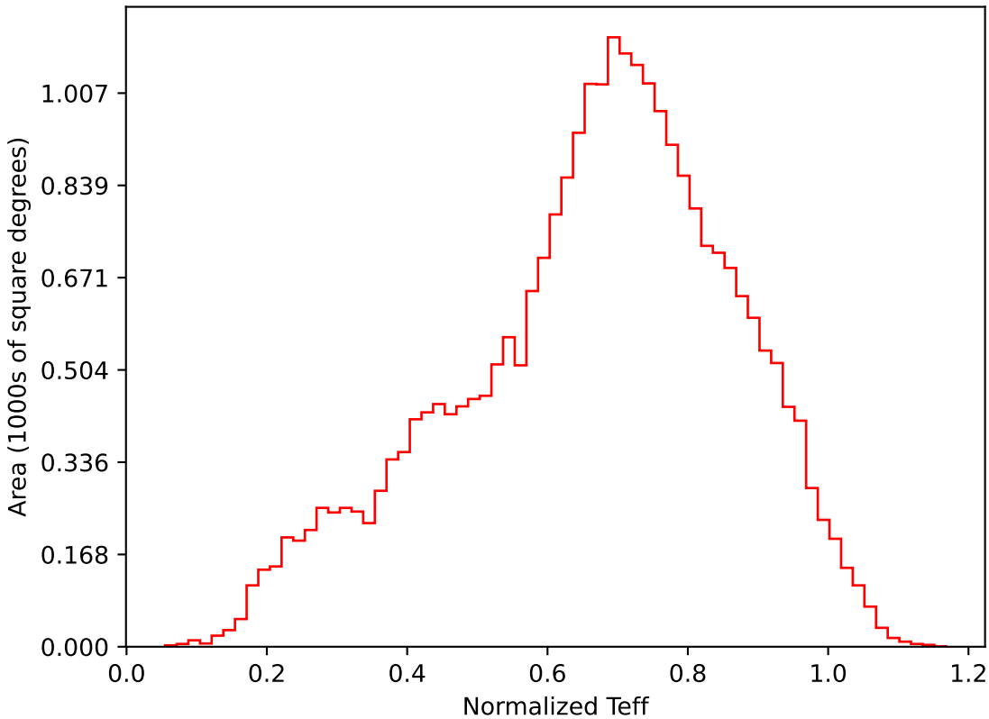
too_elab_r64_d3_ugrizy_v3.4_10yrs All sky i band: Normalized Teff
