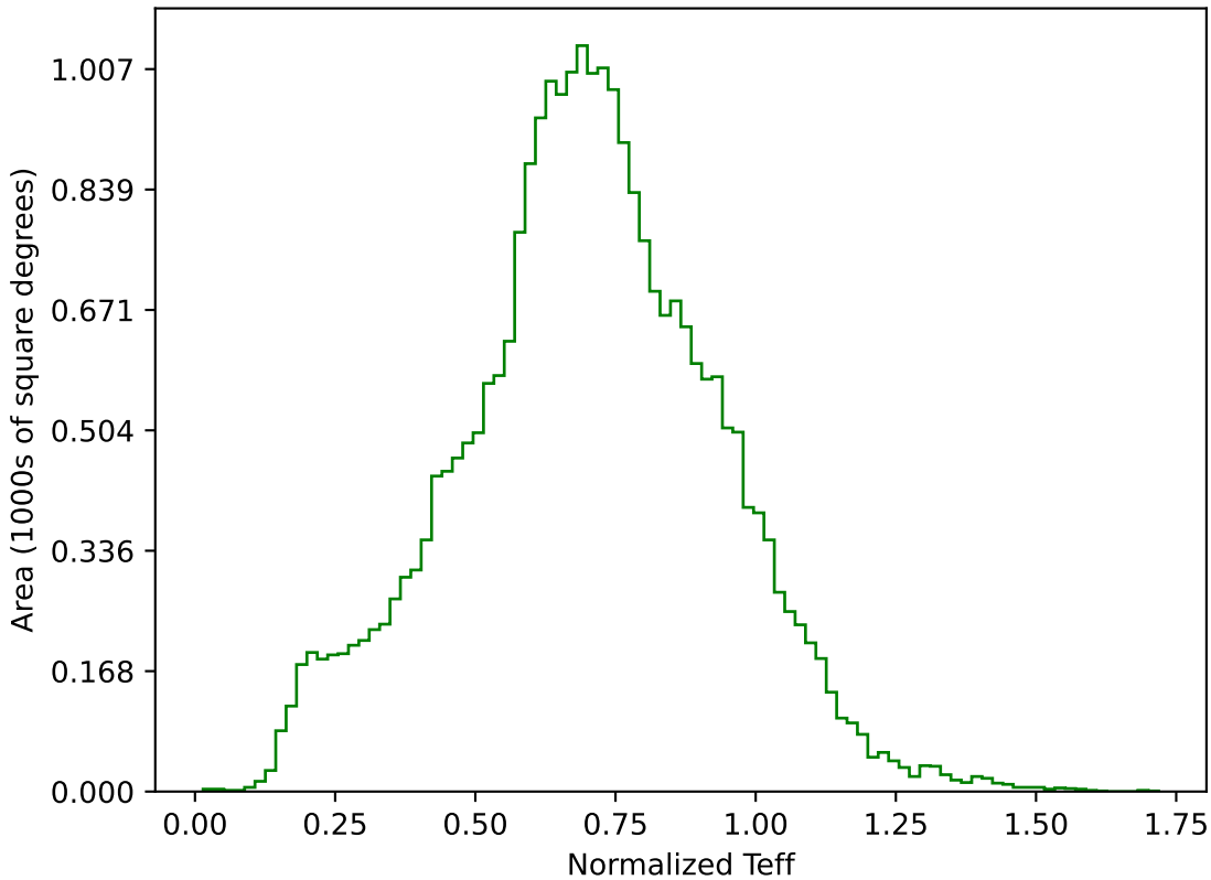
too_elab_r64_d3_ugrizy_v3.4_10yrs All sky g band: Normalized Teff
