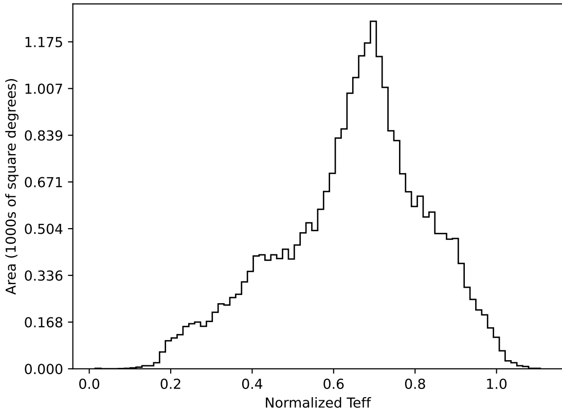
too_elab_r64_d3_ugrizy_v3.4_10yrs All sky all bands: Normalized Teff
