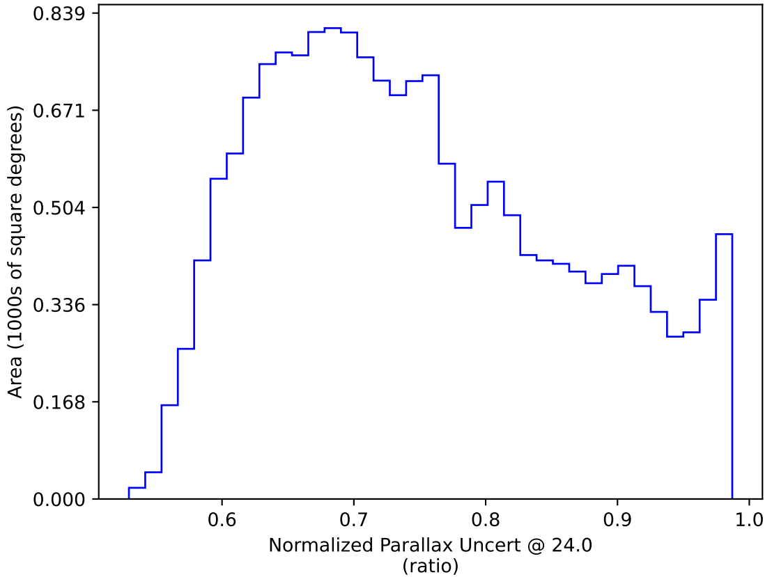
too_elab_r64_d3_ugrizy_v3.4_10yrs WFD: Normalized Parallax Uncert @ 24.0
