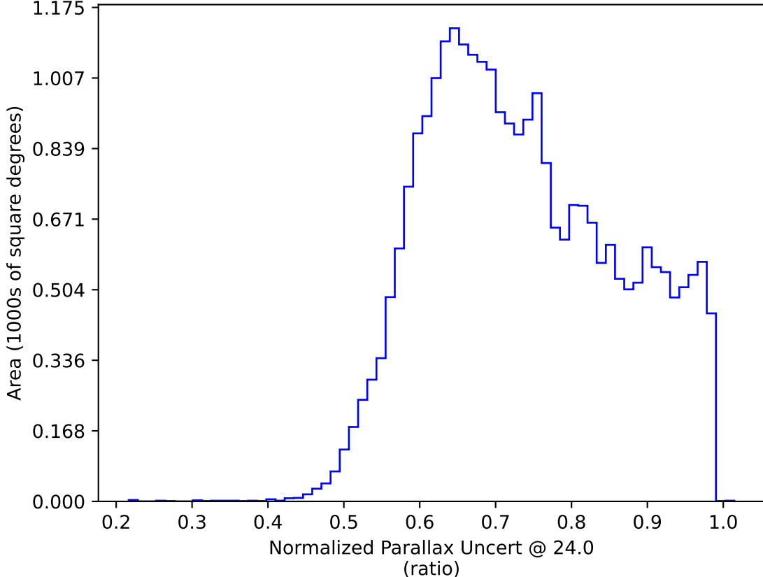
too_elab_r64_d3_ugrizy_v3.4_10yrs All sky: Normalized Parallax Uncert @ 24.0
