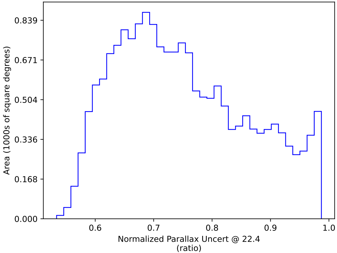
too_elab_r64_d3_ugrizy_v3.4_10yrs_WFD: Normalized Parallax Uncert @ 22.4
