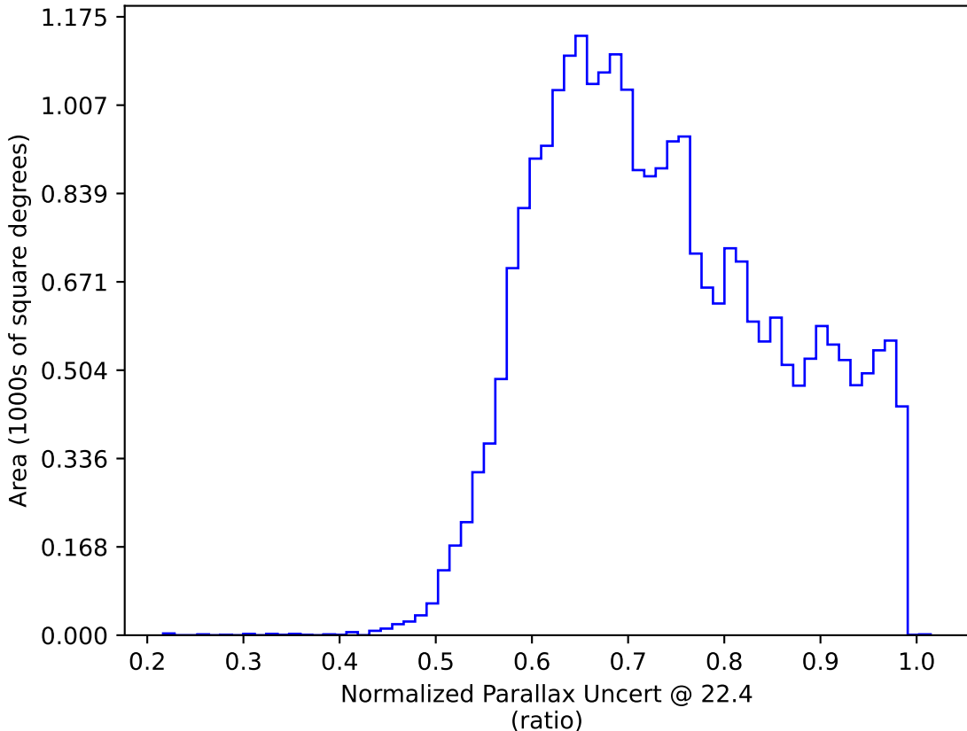
too_elab_r64_d3_ugrizy_v3.4_10yrs All sky: Normalized Parallax Uncert @ 22.4
