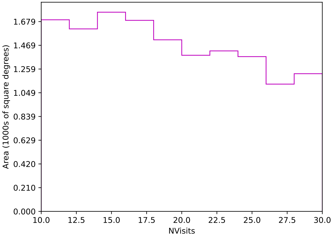
too_elab_r64_d3_ugrizy_v3.4_10yrs Yr 3-4 z band: NVisits
