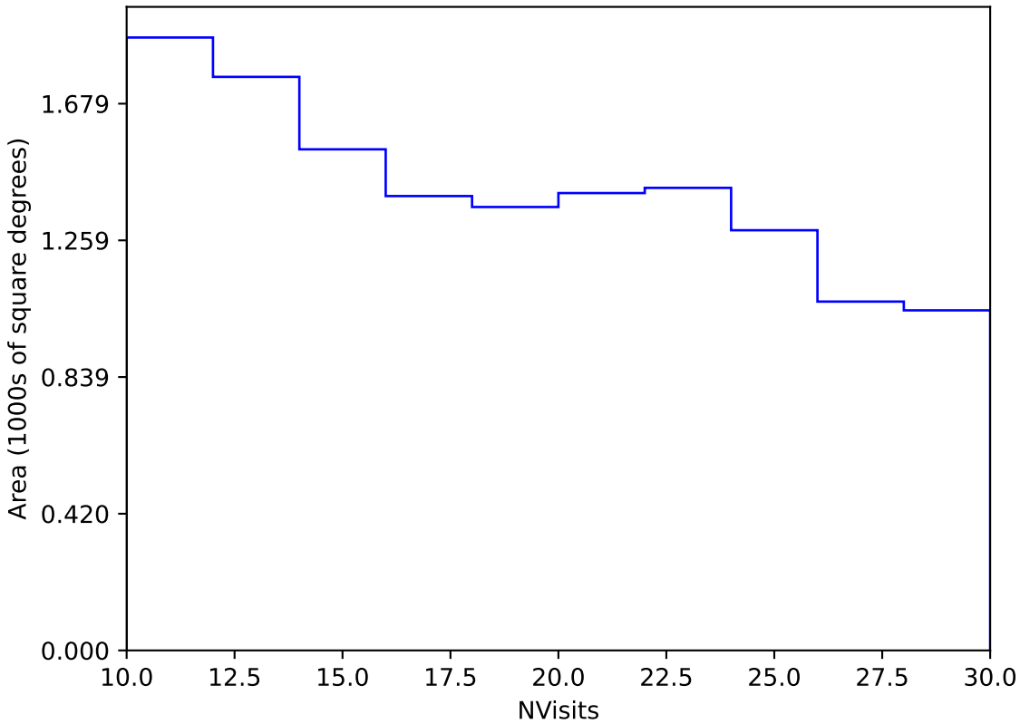
too_elab_r64_d3_ugrizy_v3.4_10yrs Yr 3-4 y band: NVisits
