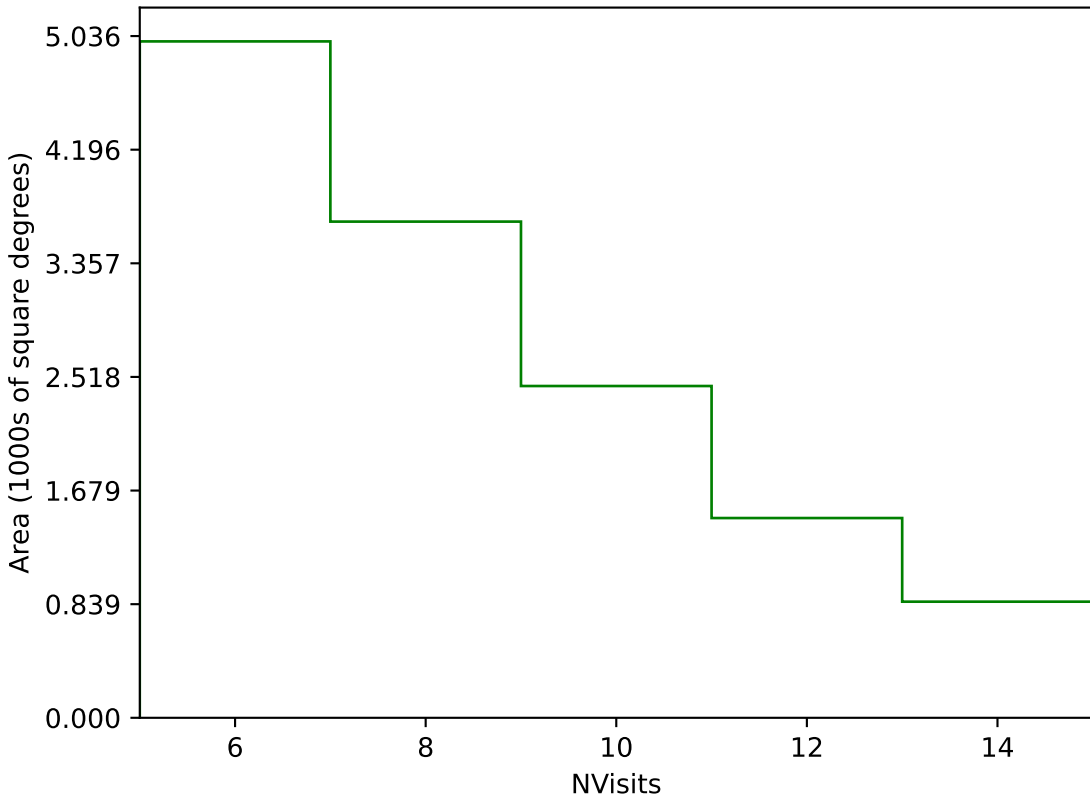
too_elab_r64_d3_ugrizy_v3.4_10yrs Yr 3-4 g band: NVisits
