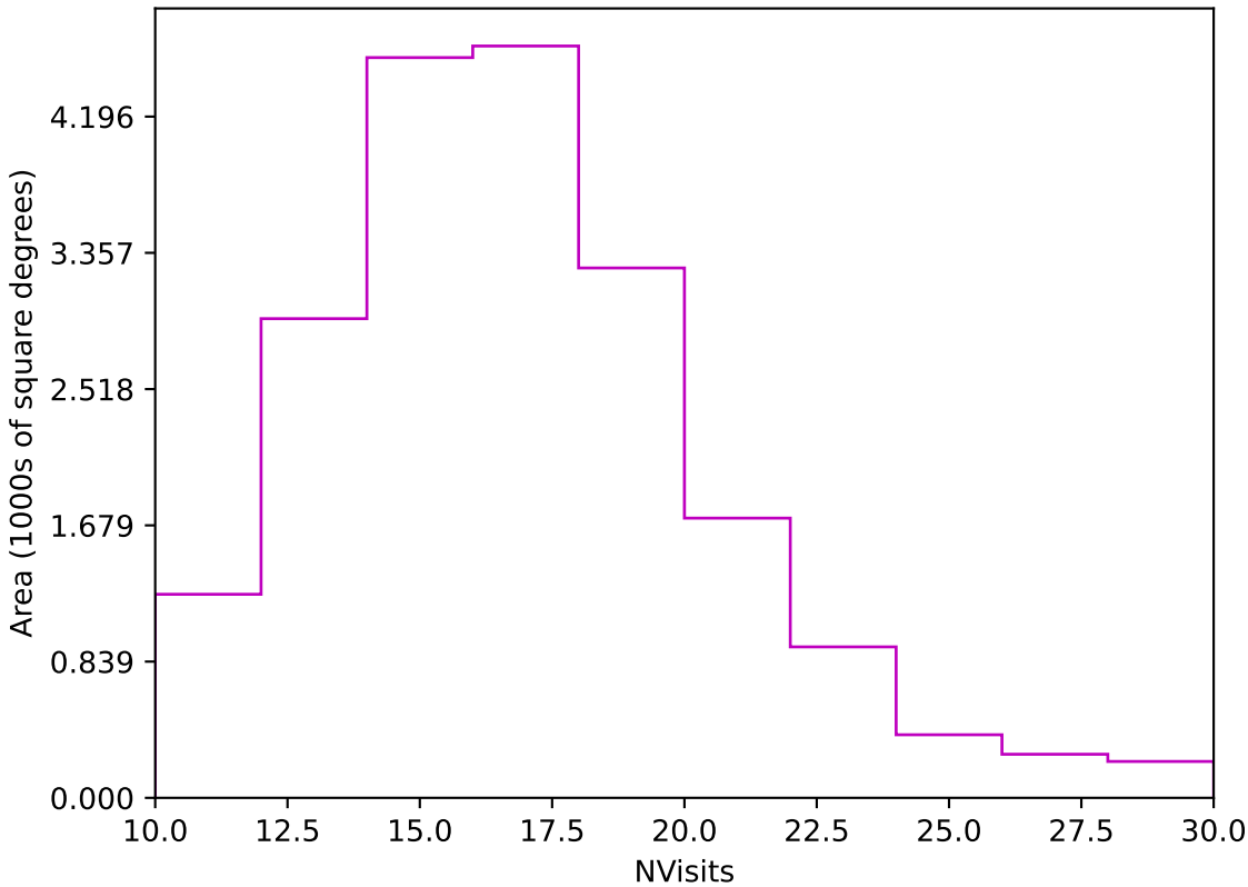
too_elab_r64_d3_ugrizy_v3.4_10yrs Yr 1 z band: NVisits
