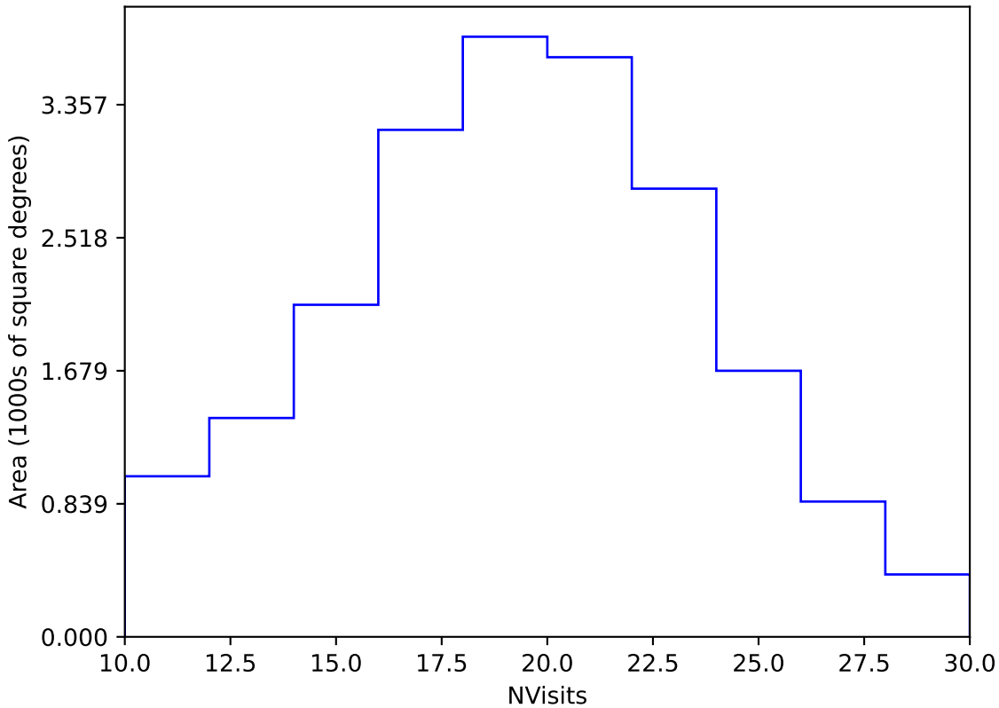
too_elab_r64_d3_ugrizy_v3.4_10yrs Yr 1 y band: NVisits
