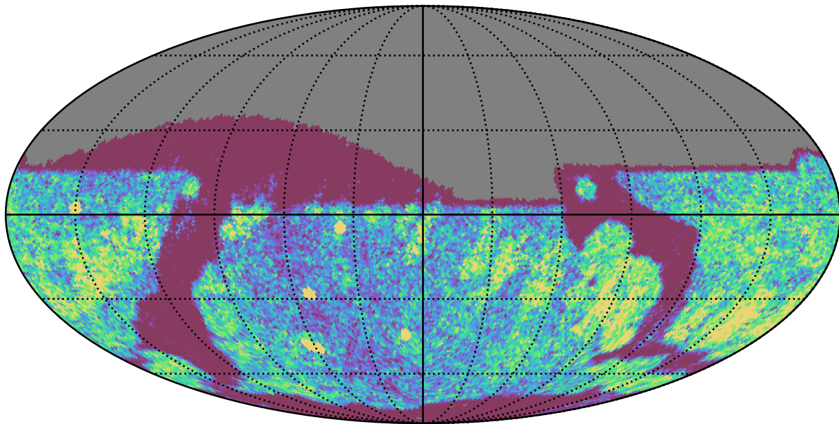
too_elab_r64_d3_ugrizy_v3.4_10yrs Yr 1 r band: NVisits
