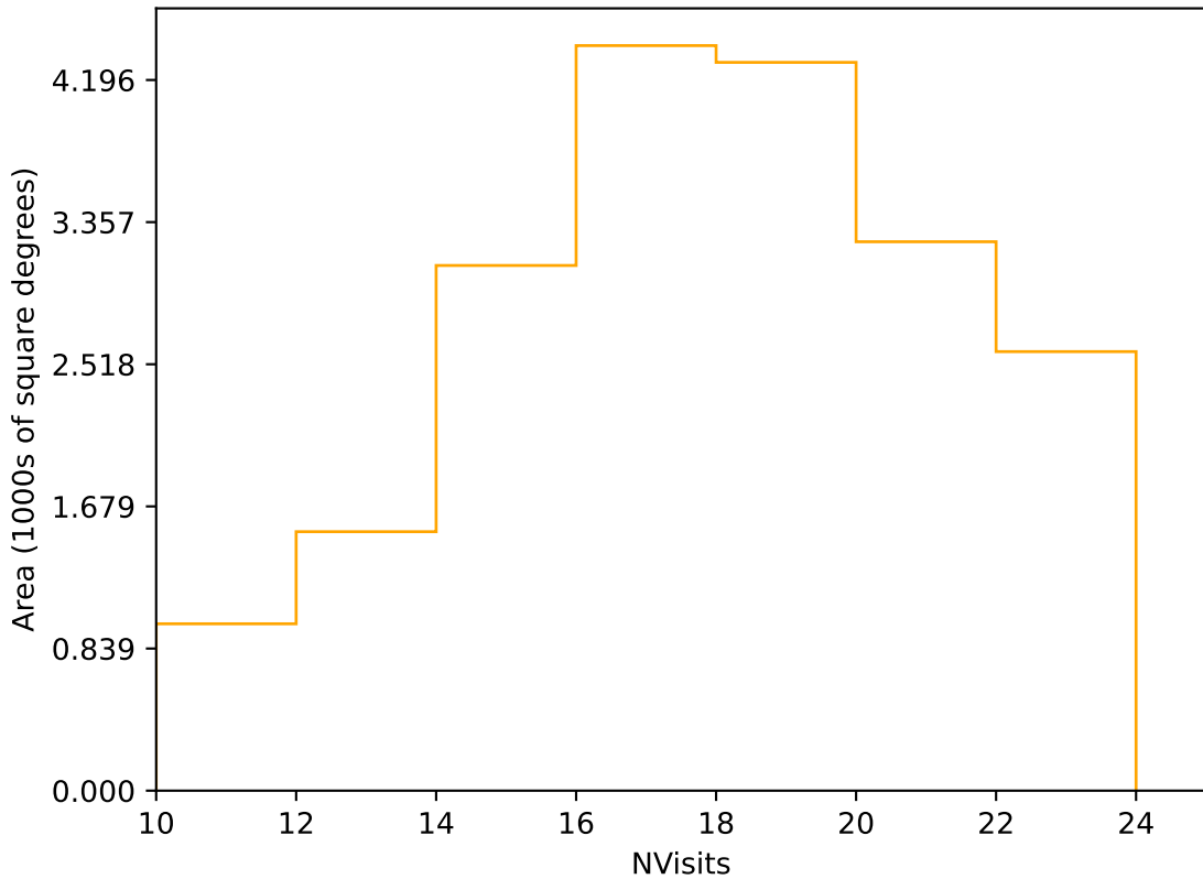
too_elab_r64_d3_ugrizy_v3.4_10yrs Yr 1 r band: NVisits
